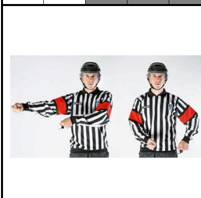
Hooking - HOOK
